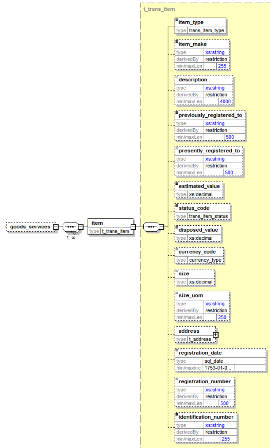
Figure 9: Overview subnode goods_services
