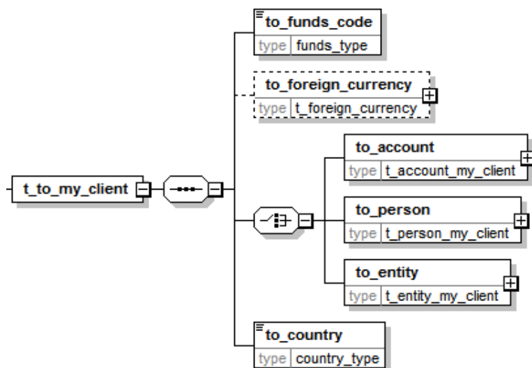
Figure 7: node t_to_my_client
